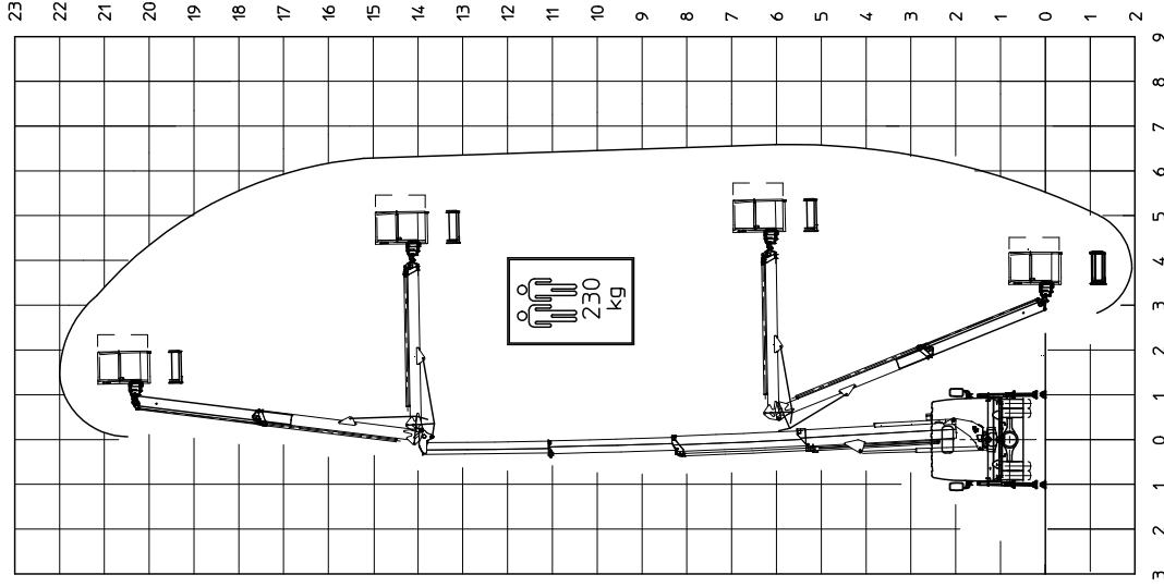
TRAVERSE IN SAGOMA - OUTRIGGER IN
